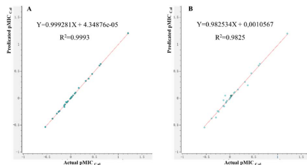
Fig. 4 Calculated \text{pMIC}_{\text{C.al}} and experimental \text{pMIC}_{\text{C.al}} values for target compounds obtained by PLS analysis using CoMFA (A) and CoMSIA (B) models.
