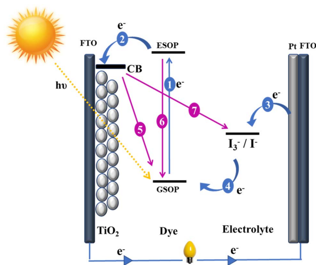
Fig. 4 Working mechanism of DSSCs. The diagram shows the electron flow and energy transfer processes, where blue arrows indicate the desired pathways for efficient energy conversion, and purple arrows highlight charge recombination losses.
