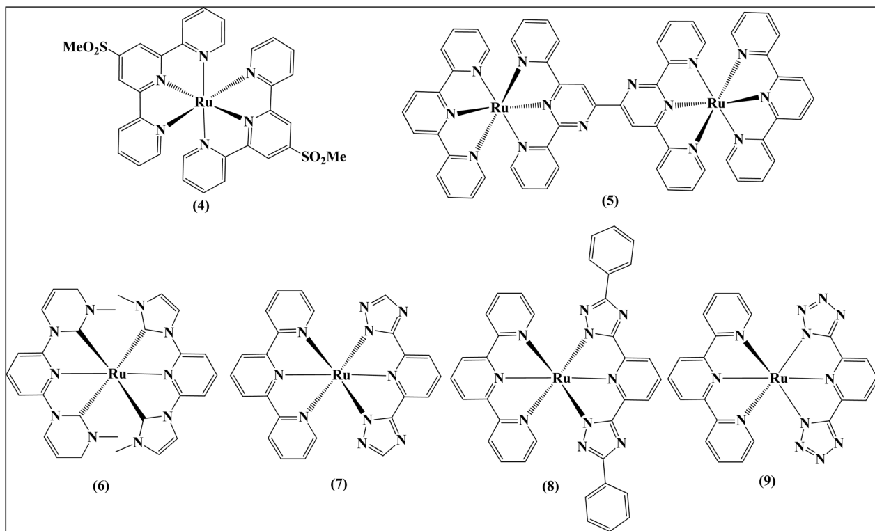
Fig. 8 Tridentate heteroleptic Ru(II) complexes (4–9).
