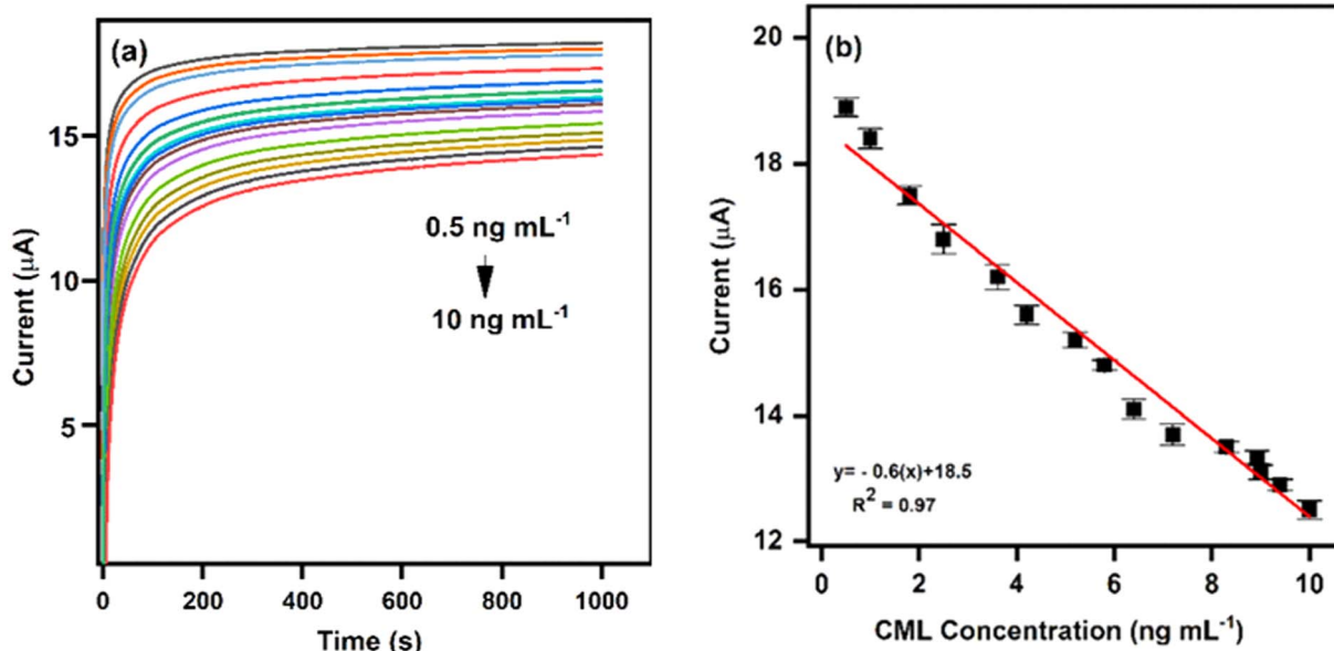
Fig. 6 (a) Amperometric current responses of the GCE/CQDs/anti-CML electrode at different CML concentrations; (b) calibration plot.
