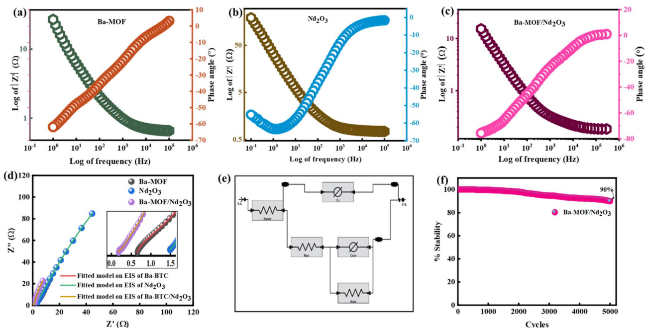
Fig. 5 (a) Bode plot of Ba-MOF. (b) Bode plot of \text{Nd}_2\text{O}_3 . (c) Bode plot of Ba-MOF/ \text{Nd}_2\text{O}_3 . (d) Nyquist plot of fabricated electrodes with its zoomed part in the inset. (e) Fitted model circuit. (f) Cyclic stability of the composite.
