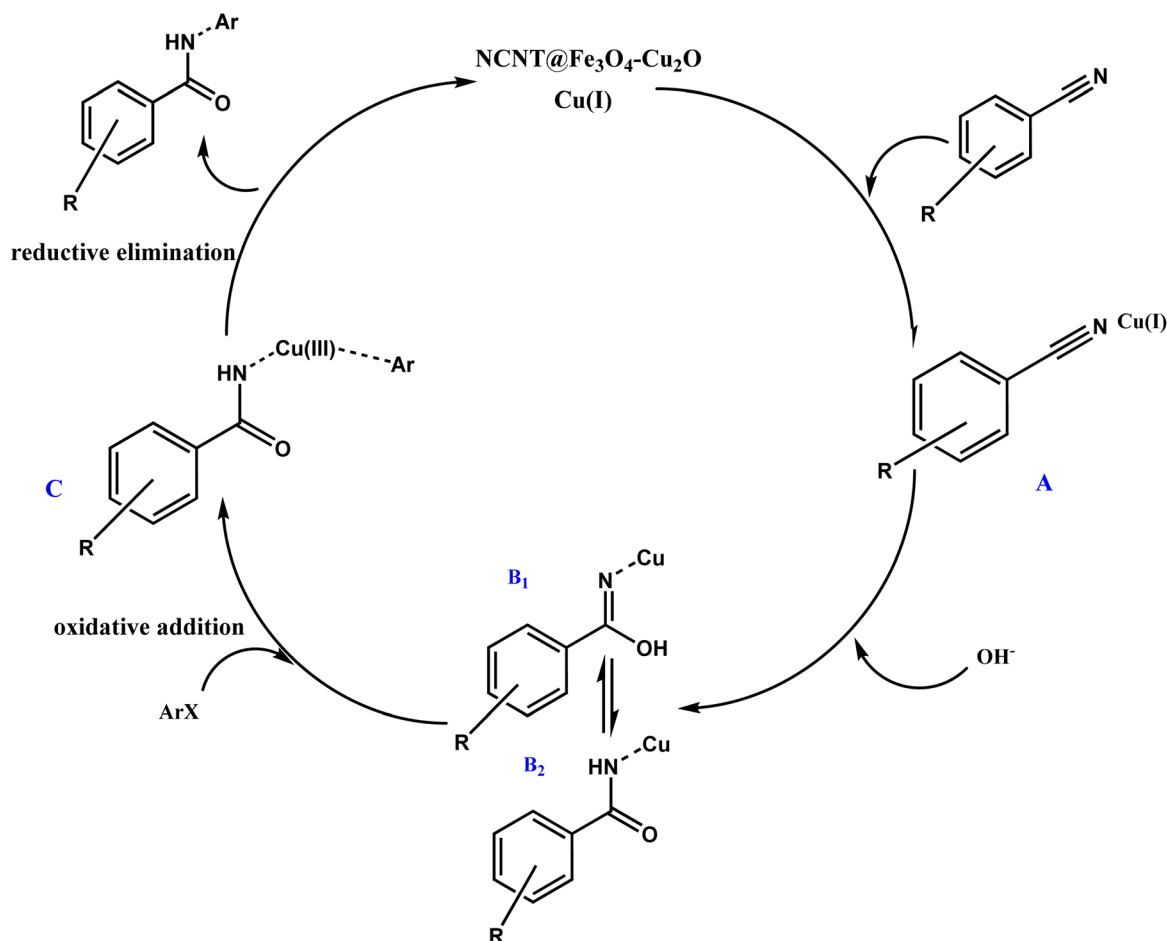
Scheme 2 Mechanism of the N -arylbenzamides synthesis.
