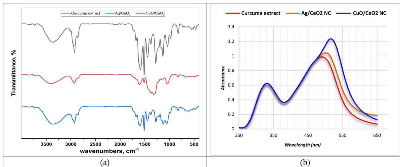
Fig. 2 FTIR spectra and UV-visible spectroscopy of the tested samples. (a) FTIR spectra of C. longa extract, Ag/CeO 2 , and CuO/CeO 2 NCs. (b) Absorbance of the samples at different wavelengths.
