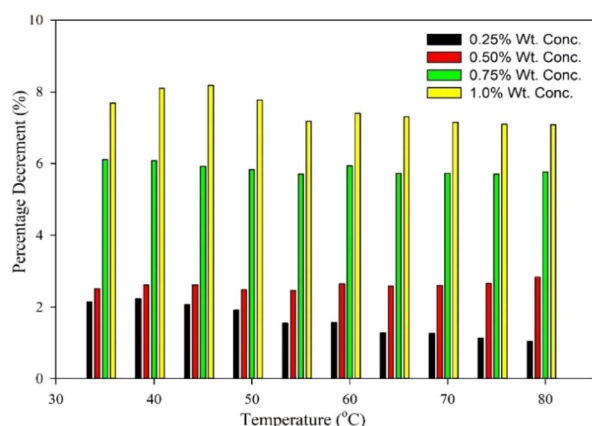
Fig. 8 Percentage decrement of the measured SHC for diamond/thermal oil nanofluids.
