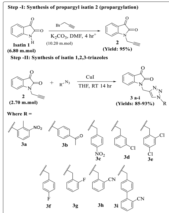
Scheme 1 General scheme for the synthesis of isatin-1,2,3-triazole derivatives (reaction conditions: step-1: propargyl bromide (1.0 mL), K 2 CO 3 , DMF, RT 4 h; step-2: CuI, THF, RT, 14 h).
