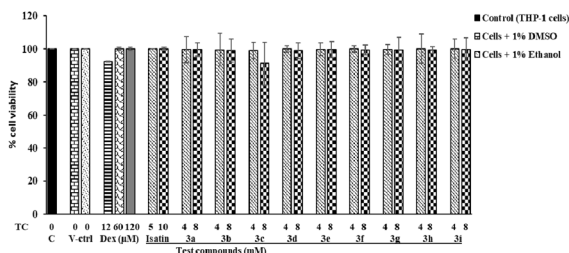
Fig. 3 MTT assay of isatin-triazole conjugates 3a–i in THP-1 cells. The viability of the cells after treatment with 4 mM and 8 mM compounds for 16 h at 37 ^{\circ}\text{C} and 5% \text{CO}_2 was determined via the MTT assay. Samples with media alone treated with compounds were used as the blanks. The data are presented as the mean \pm SD of 3 independent experiments.
