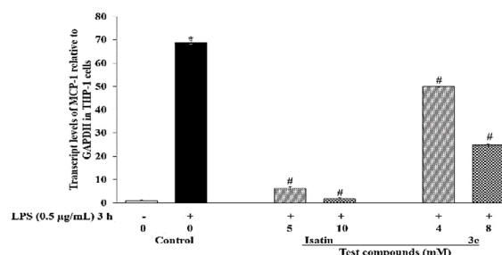
Fig. 9 Effects of the parent compound isatin and its derivative 3e on LPS-induced MCP-1 gene expression, as determined via quantitative real-time PCR. THP-1 cells were pretreated with isatin or 3e for 12 h, followed by 3 h of LPS induction. At the end of the treatment, the transcript levels of MCP-1 were quantified via real-time PCR. The data were presented as mean \pm S.D. * p < 0.001 for comparison between LPS-induced and LPS-uninduced cells, and the experiments were conducted at least three times. # p < 0.001 when comparing cells treated with LPS and test compounds to the control.
