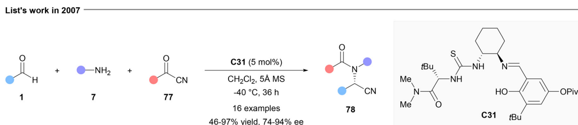
Fig. 16 Asymmetric multi-component Strecker reaction catalyzed by chiral thiourea.
