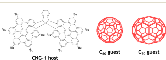
Fig. 1 All-carbon nanostructures involved in the supramolecular complexation of CNG-1 with fullerenes C_{60} and C_{70} .
