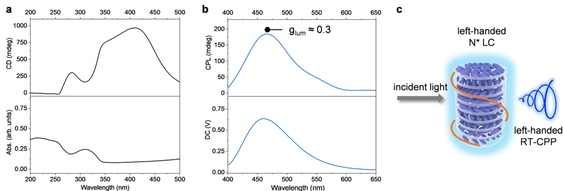
Fig. 4 Chiroptical properties and circularly polarized phosphorescence (CPP) behavior of Br10Ch in the N* phase. (a) Circular dichroism (CD, top) and UV-vis absorption (bottom) spectra of Br10Ch in the N* LC phase, confirming strong chiral ordering. (b) Circularly polarized luminescence (CPL, top) spectra with corresponding g_{lum} of Br10Ch in the N* LC phase, showing intense left-handed CPP. (c) Schematic illustration of the left-handed N* LC structure generating left-handed CPP under incident light.
