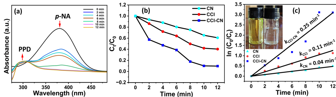
Fig. 7 (a) Time-dependent optical absorption spectra for the p -NA reduction using the CCI-CN; (b) comparison of the photocatalytic efficiencies of the CN, CCI and CCI-CN; and (c) kinetic plots for the photo-reduction of a p -NA solution using the CCI-CN under visible light irradiation.
