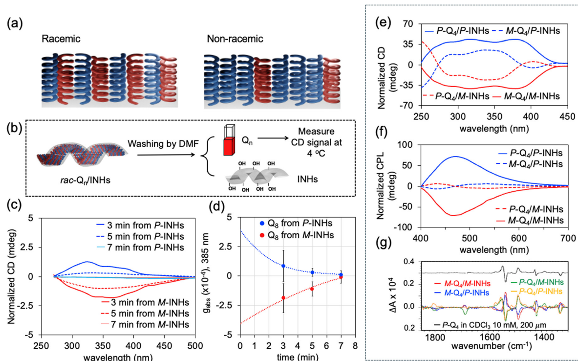
Fig. 4 (a) Illustration of the two possibilities after drop-casting rac-Q n on INHs corresponding to the relation between g_{\text{abs}} and foldamers. (b) Recovering of Q_8 from INHs by simple washing with an organic solvent. (c) ECD spectra of rac-Q 8 in DMF after removing from INHs (average from 20-time experiment). (d) Plot between g_{\text{abs}} of rac-Q 8 (at 385 nm) in function of time with the standard deviation. (e) ECD-absorption, and (f) CPL spectra of M-Q 4 /INHs and P-Q 4 /INHs ( \lambda_{\text{ex}} = 320 nm). (g) (top) VCD spectrum of P-Q 4 foldamer in \text{CDCl}_3 solution (10 mM, 200 \mu\text{m} pathlength). (bottom) Normalized differential VCD spectra of M-Q 4 /M-INHs, M-Q 4 /P-INHs, P-Q 4 /M-INHs and P-Q 4 /P-INHs samples after subtracting corresponding rac-Q 4 /P or M-INHs.
