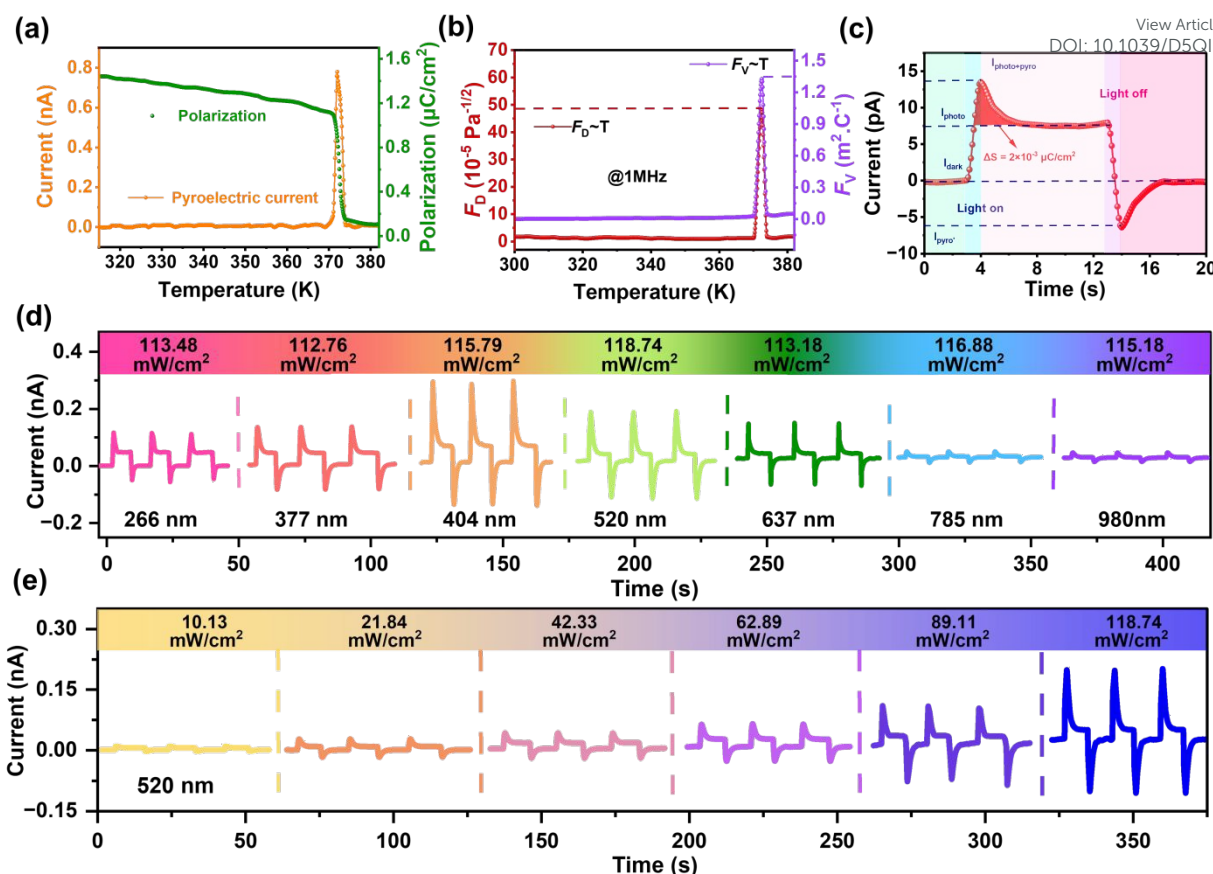
Fig. 4 a) Temperature-dependent pyroelectric currents and P_s deduced by integrating pyroelectric current. b) The simulated two FOMs of F_V and F_D . c) I-t curves measured under 404 nm irradiation at zero bias (5.44 mW cm -2 ). d) Photoactivities of 1 under light illumination of different wavelengths. e) I-t curves measured under 520 nm laser irradiation with different densities at zero bias.
