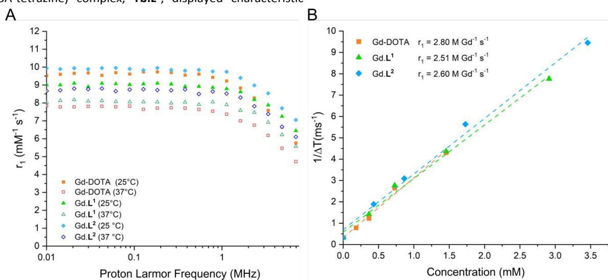
Figure 3. A) NMRD profiles for Gd complexes before and after IEDDA cycloaddition compared to Gd-DOTA, at 25 °C (solid symbols) and 37 °C (hollow symbols); B) Longitudinal relaxivity of Gd complexes at 9.4 T (400 MHz) for phantoms of 1 mL solution in PBS buffer at different concentrations at 25 °C. Concentrations corrected for Gd concentration using bulk magnetic susceptibility shifts. 73,74
