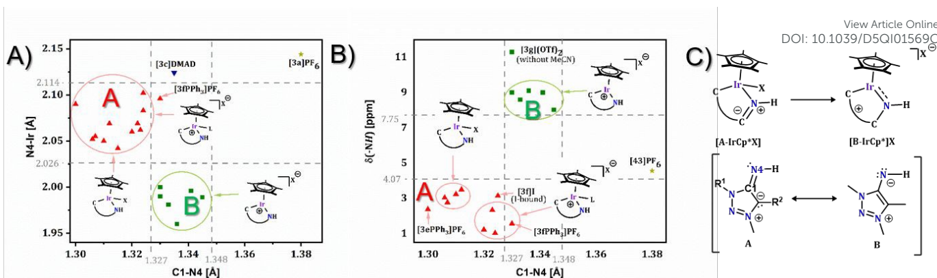
Figure 2: A) Graphical relation of the N4-Ir and the C1-N4 bond length in the IrCp*-complexes 3 . B) Graphical relation of the resonance of the -NH in the 1 H-NMR spectra and the C1-N4 bond length in the IrCp*-complexes 3 . C) Possible coordination modes in the discussed MII-IrCp* complexes.
