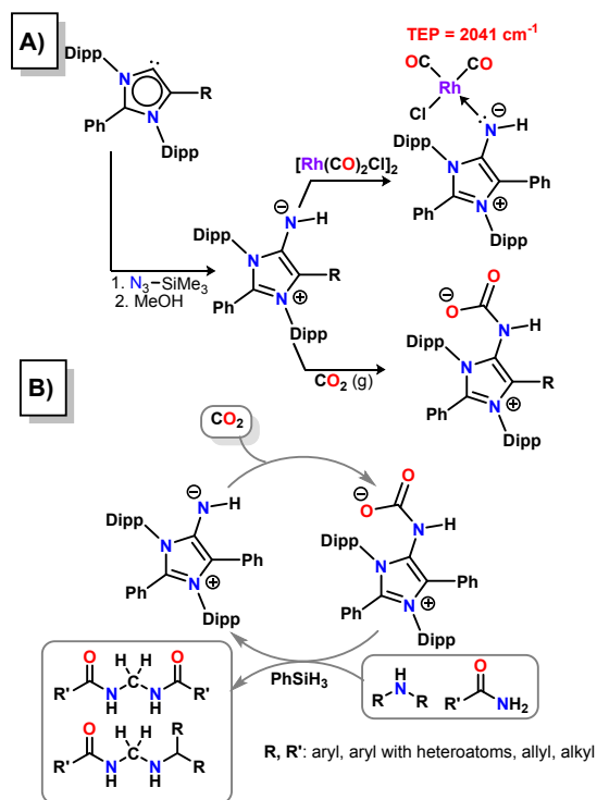
Scheme 10 A) Synthesis of aNHIs as reported by Mandal et al , the reactivity thereof with \text{CO}_2 -gas and [\text{Rh}(\text{CO})_2\text{Cl}]_2 and the respective TEP determined. B) Amide/amine-coupling with \text{CO}_2 catalysed by an aNHI. 71
