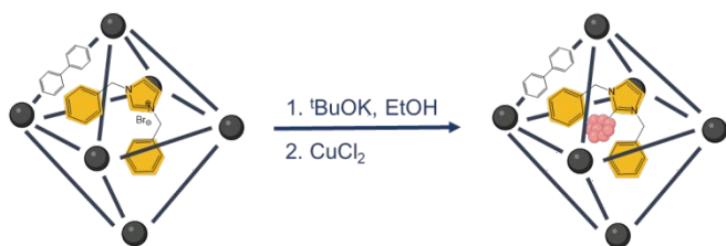
Figure 19. Synthesis reaction scheme to produce 2Bn-Cu@UiO-67 from UiO-67-NHC by addition of base and copper salt. Adapted) with permission from 88 . Copyright 2025 John Wiley and Sons.
