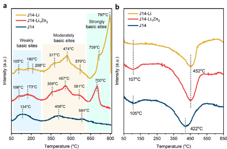
Fig. 6 Chemisorption experiment of used catalysts. (a) \text{CO}_2 -TPD and (b) \text{H}_2 -TPD plots of used J14-Li, J14-Li _1 Zn _3 , and J14.
