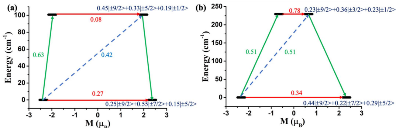
Fig. 7 The mechanism of magnetization relaxation of (a) [\text{U}(\text{Tp}^{\text{Me}_2})_2(\text{THF})_2] ( 7 ) and (b) [\text{U}(\text{Tp}^{\text{Me}_2})_2\text{CH}_2\text{Ph}] ( 9 ). The red arrows denote the QTM via the ground state and TA-QTM via the first excited state. The sky-dotted arrow represents the Orbach process. The green arrows indicate the most possible pathway of magnetisation relaxation.
