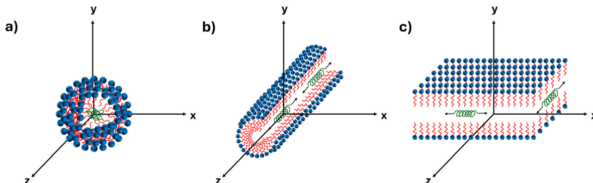
Fig. 9 Direction of monomer propagation inside (a) cubic, (b) hexagonal, and (c) planar micelles.
