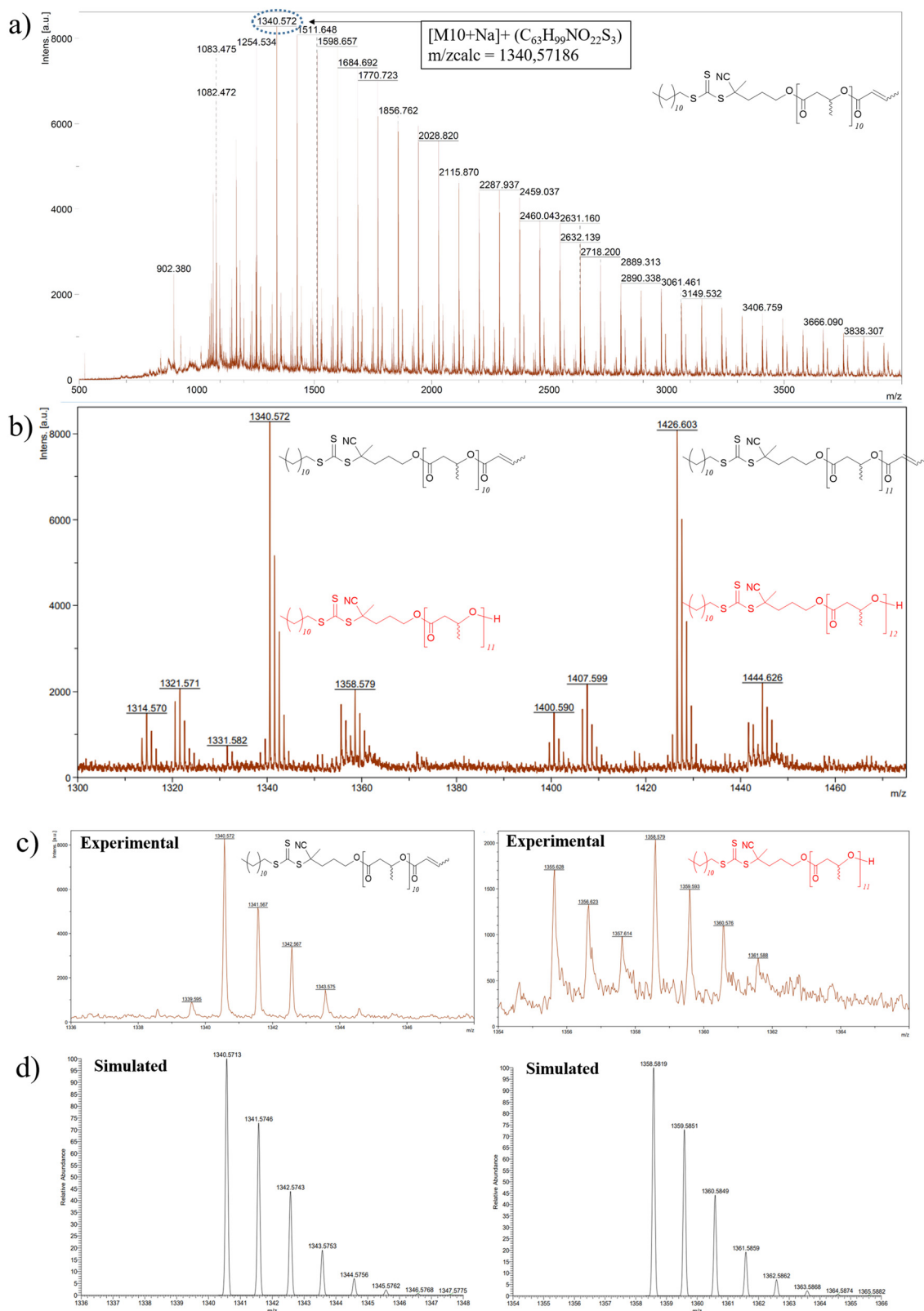
Fig. 3 (a) High resolution MALDI-ToF mass spectrum (DCTB matrix, ionized by Na^+ ), of PHB 83 -TTC prepared by ROP of racemic \beta -butyrolactone catalyzed by Y(ONNO^{Me})_3 and initiated by TTC-OH (Table 1, entry 1). The lower molar mass macromolecules are observed with m/z experimental ( m/z_{exp} ) vs. calculated ( m/z_{calc} ) values, respectively, for the crotonate-PHB 83 -TTC for: DP = 9: 1254.534 vs. 1254.535; DP = 10: 1340.572 vs. 1340.572; DP = 11: 1426.603 vs. 1426.609; DP = 20: 2200.909 vs. 2200.939, (b) zoom and assignment of the two major populations crotonate-PHB 83 -TTC and HO-PHB 83 -TTC, (c) zoom of the major population crotonate-PHB 83 -TTC (DP = 10 and DP = 11) and the minor population HO-PHB 83 -TTC (DP = 11 and DP = 12), (d) simulation of the above major and minor populations, respectively.
