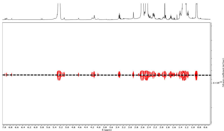
Fig. 2 DOSY NMR spectrum (500 MHz, \text{CDCl}_3 , 25 ^\circ\text{C} ) of \text{PHB}_{83}\text{-TTC} prepared by ROP of racemic \beta -butyrolactone catalyzed by Y\{ONNO^{Me}\} and initiated by TTC-OH (Table 1, entry 1).
