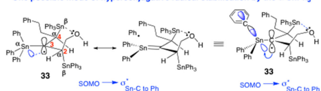
Fig. 3 The \alpha - \text{Ph}_3\text{Sn} SOMO \rightarrow \sigma^*_{\text{Sn-C(Ph)}} delocalising stabilisation of 33 .
