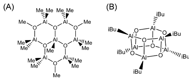
Fig. 1 Experimentally determined molecular models of MAO based on: (A) isolation from an MAO solution by Atwood et al. 16 and (B) isolation from isobutylaluminoxane by Barron et al. 17
