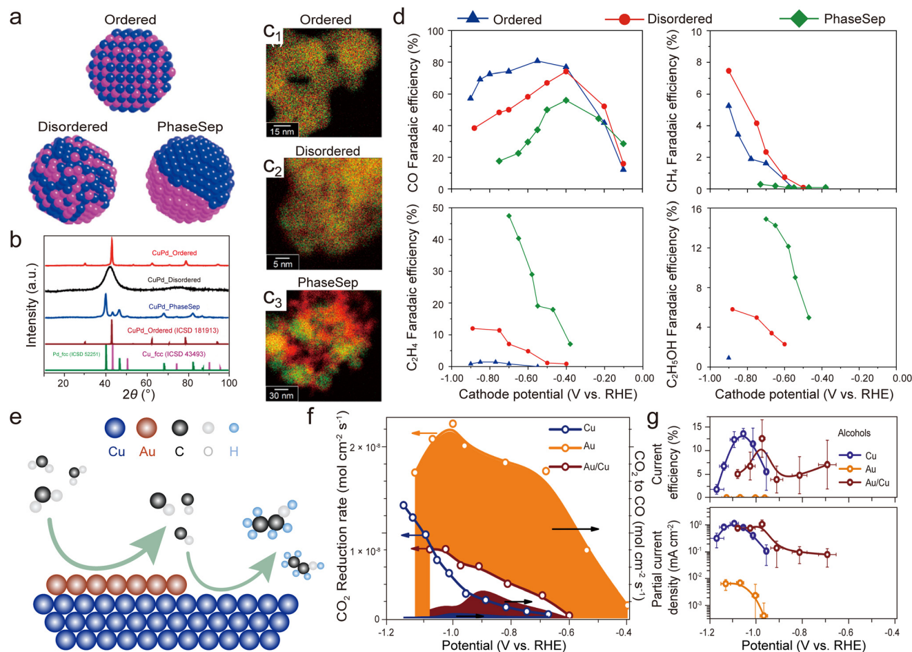
Fig. 3 (a and b) Schematic of Cu–Pd nanoalloys with ordered, disordered, and phase-separated structures, along with their corresponding XRD spectra. ( C_1 – C_3 ) EDS elemental mapping of three distinct Cu–Pd nanoalloys with ordered, disordered, and phase-separated structures, respectively, showing Cu (red) and Pd (green). (d) FEs of CO, CH_4 , C_2H_4 , and C_2H_5OH under three distinct structural configurations. (e) Schematic of CO_2RR over CuAu hybrid with a phase-separated state. (f) CO_2 consumption and CO_2 production rate as a function of applied potential. (g) Current efficiency and partial current density of alcohols in CO_2 reduction products corresponding to Cu, Au, and CuAu hybrids. (a–d) Reprinted with permission from Kenis et al. 26 Copyright 2017, the American Chemical Society. (f–g) Reprinted with permission from Jaramillo et al. 27 Copyright 2018, Springer Nature.
