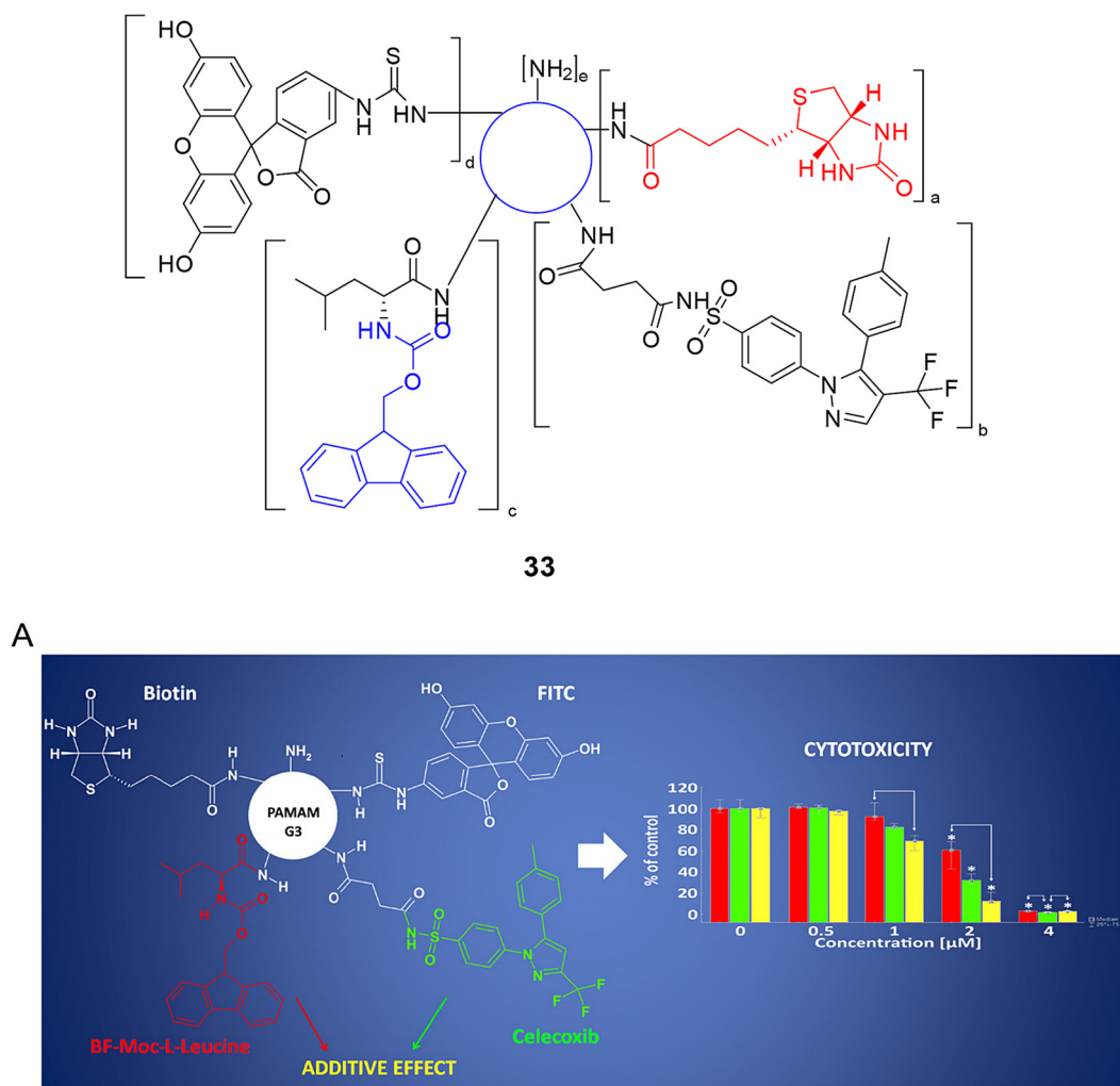
Fig. 24 The structure of compound 33. Schematic formulae of studied conjugates: G3^{1B31C} ( a = 1, b = 31, c, d, e = 0 ); G3^{1B31L} ( a = 1, c = 31, b, d, e = 0 ); G3^{1B16C15L} ( a = 1, b = 16, c = 15, d, e = 0 ); G3^{1B20C1F} ( a = 1, b = 20, c = 0, d = 1, e = 10 ); G3^{1B20L1F} ( a = 1, b = 0, c = 20, d = 1, e = 10 ); G3^{1B10C10LF} ( a = 1, b = 10, c = 10, d = 1, e = 10 ). (A) Drugs and their effects on cell viability. Reproduced with permission. 99 Copyright 2018, Elsevier.
