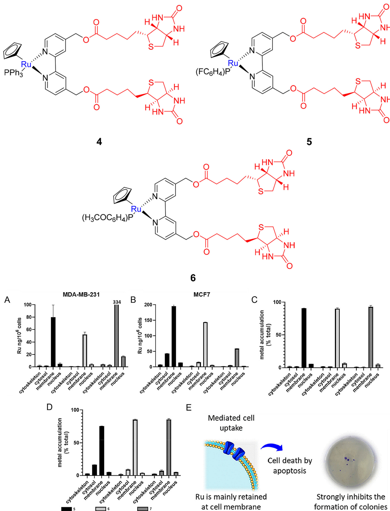
Fig. 6 Chemical structures of compounds 4, 5 and 6. (A–D) Distribution of Ru in cells after drug treatment. (E) Representative images of colony formation assay. Reproduced with permission. 39 Copyright 2019, ACS.
