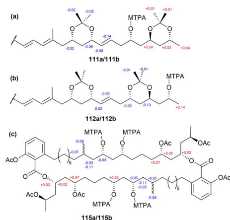
Fig. 61 Chemical shift differences ( \Delta\delta_{S-R} ) between ( S )- and ( R )-MTPA esters. (a) Partial assignment of ( S )- and ( R )-MTPA esters ( 111a/111b ). (b) Partial assignment of ( S )- and ( R )-MTPA esters ( 112a/112b ). (c) Assignment of ( S )- and ( R )-MTPA esters ( 115a/115b ).
