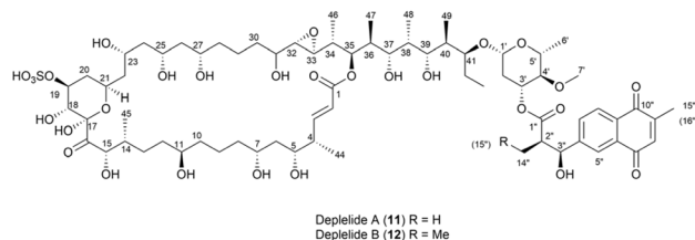
Fig. 9 Structures of deplelides A (11) and B (12).
