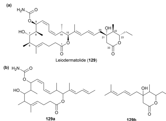
Fig. 76 (a) Structure of leiodermatolide (129). (b) Model structures 129a and 129b used in DP4 calculations for the macrolactone and δ-lactone parts, respectively.
