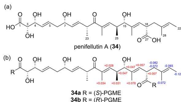
Fig. 23 (a) Structure of penicillutin A ( 34 ) and (b) \Delta\delta_{S-R} values of the PGME derivatives ( 34a and 34b ) of 34 .
