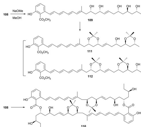
Fig. 59 Methanolysis and acetonide formation of marinomycin A ( 108 ).
