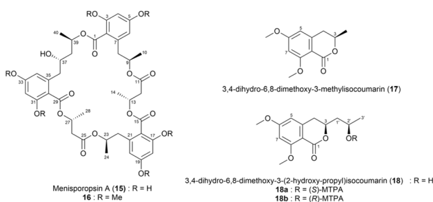
Fig. 12 Structures of menisporopsin A (15), its methylated derivative (16), 3,4-dihydro-6,8-dimethoxy-3-methylisocoumarin (17), 3,4-dihydro-6,8-dimethoxy-3-(2-hydroxy-propyl)isocoumarin (18), and the (S)- and (R)-MTPA esters of 18 (18a and 18b).
