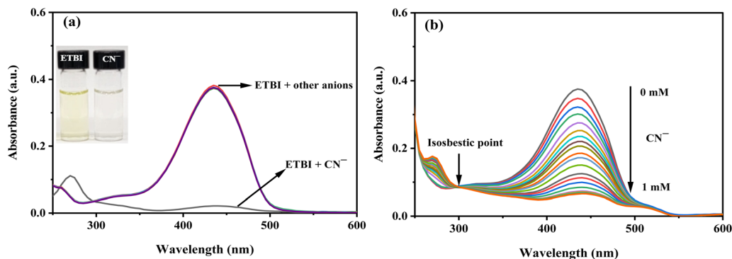
Fig. 1 (a) UV/Vis absorption spectra of ETBI (10 \mu M) in the presence of 10 equivalents of different anions in DMSO/H 2 O (1 : 9, v/v, 0.1 M HEPES; pH = 7.0). (b) titrated with \text{CN}^- ion DMSO/H 2 O (1 : 9), v/v, 0.1 M HEPES; pH = 7.0.
