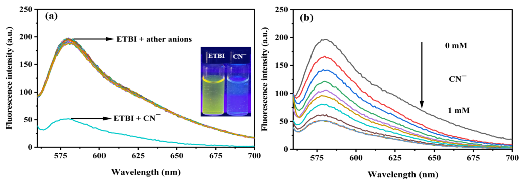
Fig. 2 Fluorescence spectra of ETBI (50 \mu M) (a) in the presence of 10 equivalents of anions (b) titrated with \text{CN}^- ion DMSO/H 2 O (1 : 1), v/v, 0.1 M HEPES buffer, \lambda_{\text{ex}} = 540 nm.
