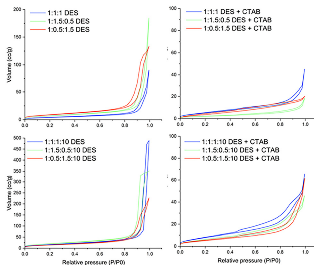
Fig. 5 \text{N}_2 adsorption/desorption isotherms at 77 K for iron oxide samples post-calcination made from the solvothermal synthesis in ChCl:U:Gly:W DES and ChCl:U:Gly:W DES, with and without added CTAB.
