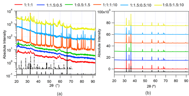
Fig. 4 PXRD from zinc-containing samples made from the solvothermal synthesis in ChCl:U:Gly DES with added CTAB at different solvent compositions (red trace – 1:1:1 DES, blue trace – 1:1.5:0.5 DES, green trace – 1:0.5:1.5 DES, orange trace – 1:1:1:10 DES, cyan trace – 1:1.5:0.5:10 DES and yellow trace – 1:0.5:1.5:10 DES). (a) PXRD from the samples pre-calcination, and (b) PXRD from samples post-calcination. The black traces show the JCPDS XRD patterns of the corresponding compounds: (a) solid black trace zinc carbonate ( \text{ZnCO}_3 ; JCPDS 8-449) and dashed black trace zinc carbonate hydroxide ( \text{Zn}_5(\text{CO}_3)_2(\text{OH})_6 ; JCPDS 19-1458); (b) solid black trace hexagonal wurtzite structure of ZnO (JCPDS 36-1451).
