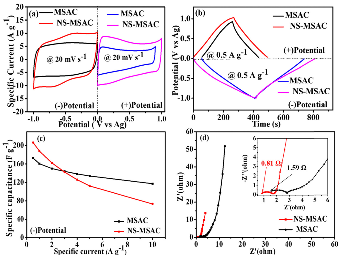
Fig. 3 (a) CV curves at 20 mV s -1 , (b) GCD curves at 0.5 A g -1 , (c) specific capacitance vs. specific current, (d) Nyquist plot for MSAC and NS-MSAC samples.
