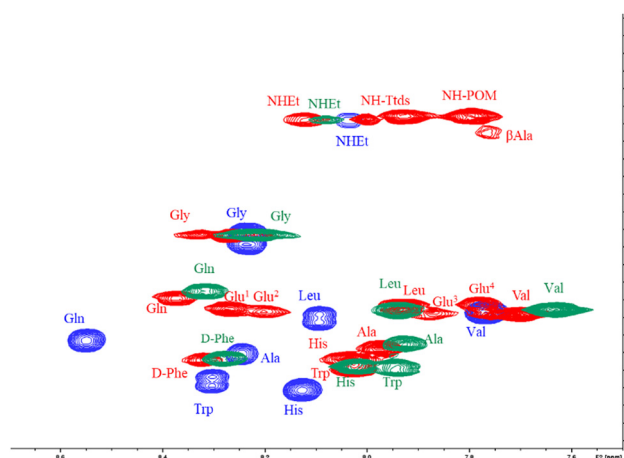
Fig. 4 Overlaid COSY spectra (in d_6 -DMSO) for NH- \text{CH}\alpha cross peaks belonging to free and V_6 -grafted DB (Pep-1 (blue), POV-1 (green) and POV-4 (red)). The spectra were acquired on a Bruker DMX-600 instrument operating at 599.90 MHz for ^1\text{H} at 298 K.
