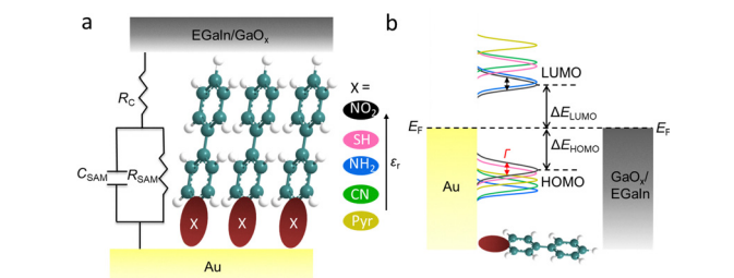
Fig. 1 (a) Schematic illustration of the Au-X(C_6H_4)_nH/GaO_x/EGaIn junction with n = 1 or 2 and X = -NO_2 , -SH , -NH_2 , -CN , and -Pyr where “—” indicates covalent bond, “//” indicates the non-covalent contact and “//” represents the physical phase between GaO_x and EGaIn . In all experiments, the bottom gold electrode was grounded, while the voltage was applied to the top EGaIn electrode. (b) The proposed energy level alignment of the SAMs embedded in Au and GaO_x/EGaIn leads was based on our experimental results. The coupling strength between molecule and electrode \Gamma (schematically indicated by changes in the width given by the double arrow in red), \Delta E_{HOMO} , and \Delta E_{LUMO} (given by the double arrows in black) of the SAMs in the junction vary with X.
