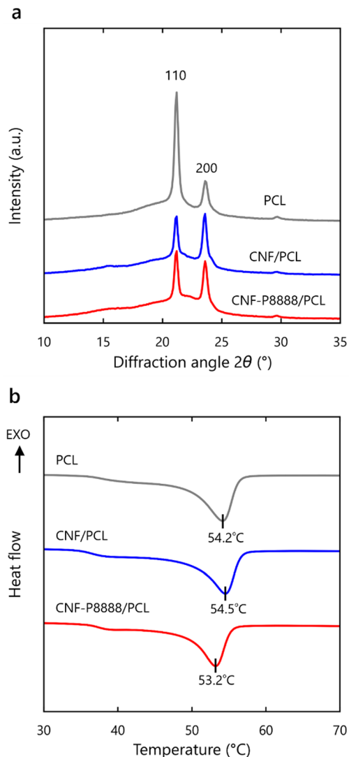
Fig. 4 Crystallinity analyses. (a) XRD profiles and (b) DSC curves of pristine PCL, CNF-P8888/PCL, and CNF/PCL at 10% w/w CNF content.
