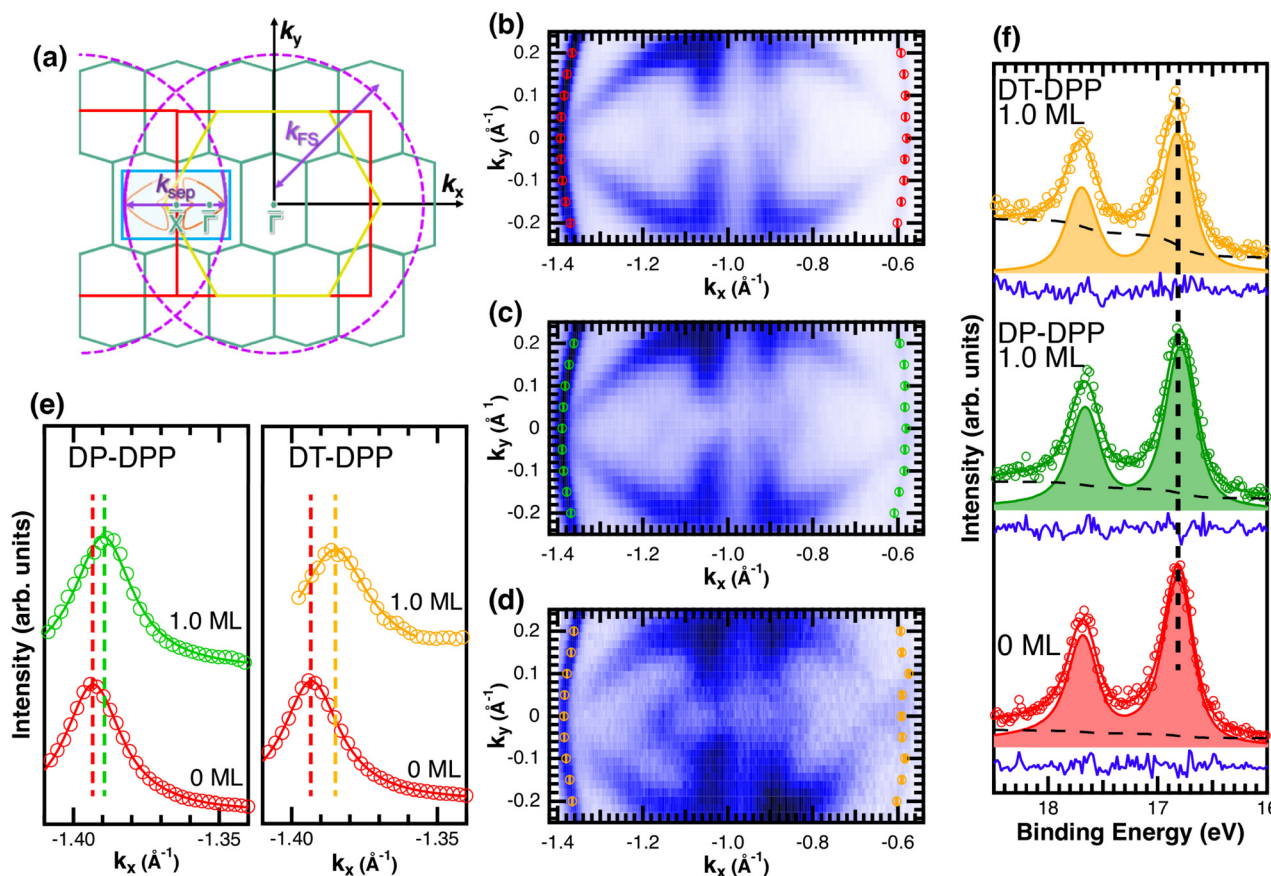
Fig. 3 ARPES results. The Brillouin zones (BZs) and schematic FSs are shown in (a). The (\sqrt{7} \times \sqrt{3}) BZ, the Si(111)-(1 × 1) BZ, and the idealized (1 × 1) BZ of the In layer are indicated by green lines, yellow lines, and red lines, respectively. The violet dashed lines and the orange lines are the circular-shaped FSs and butterfly-shaped FSs of Si(111)-In( \sqrt{7} \times \sqrt{3} ). The blue rectangle indicates the area of the FSs measured using ARPES. K_F is the radius of the circular-shaped FS, and K_{sep} is the distance between two circular-shaped FSs that we measured to discuss the amount of charge doping. (b) shows the FS of a pristine Si(111)-In( \sqrt{7} \times \sqrt{3} ) surface, and (c) and (d) are the FSs of Si(111)-In( \sqrt{7} \times \sqrt{3} ) fully covered by DP-DPP and DT-DPP, respectively. The open circles in (b)–(d) mark positions of the circular-shaped FSs obtained by MDCs measured at different k_y . (e) shows the MDCs of the circular-shaped FSs of a pristine and DP-DPP and DT-DPP covered Si(111)-In( \sqrt{7} \times \sqrt{3} ). The MDCs were obtained by the summation of the photoelectron intensity within a k_y range of 0 \pm 0.025 \text{ \AA}^{-1} . The open circles are the experimental data, and the solid lines overlapping them show the Lorentzian fittings. (f) In 4d core-level spectra of pristine (bottom), DP-DPP (middle) and DT-DPP (top) covered surfaces.
