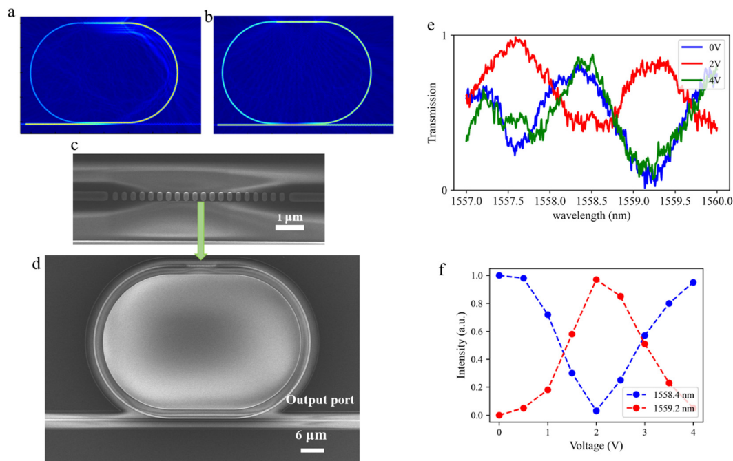
Fig. 4 LC meta-waveguide phase shifter in an MRR. (a) and (b) Two switching states of the MRR in simulation. (c) and (d) SEM images of the metawaveguide and MRR. (e) The spectrum of the MRR at wavelengths ranging from 1557 nm to 1560 nm under 0 V, 2 V, and 4 V applied voltages. (f) The transmission variation of the MRR at wavelengths of 1558.4 nm and 1559.2 nm as the voltage is applied from 0 V to 4 V.
