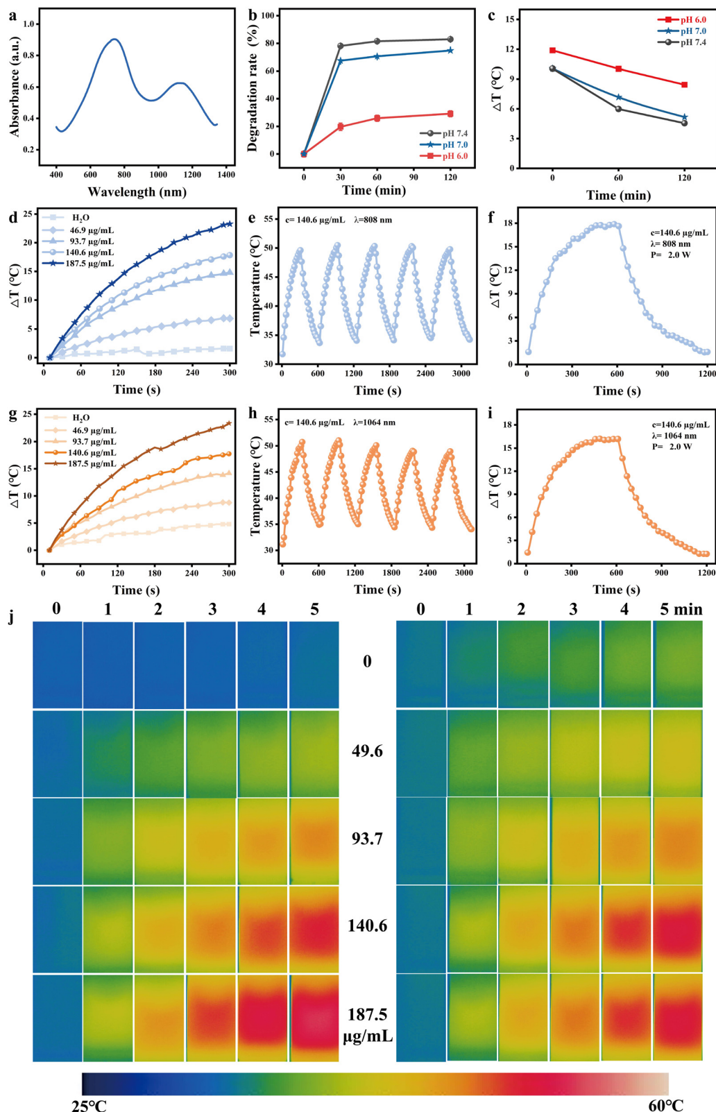
Fig. 2 Photothermal performance of PMB. (a) UV-vis absorption spectrum of PMB. (b) The degradation rate of PMB (140.6 \mu\text{g mL}^{-1} 1 mL) in different pH (6.0, 7.0, 7.4) Saline and (c) temperature rise curves after degradation (808 nm 1.5 W, 5 min). Photothermal heating curves of PMB aqueous suspensions (1 mL) with different concentrations under the irradiation of (d) 808 nm (g) 1064 nm lasers. Photothermal stability of PMB aqueous suspensions (1 mL) under (e) 808 nm and (h) 1064 nm lasers through repeated heating and cooling measurements. Heating of PMB aqueous suspensions (1 mL) with (f) 808 nm and (i) 1064 nm laser irradiation for 10 min and then cooling at ambient environment; (j) thermal imaging of PMB under (left) 808 nm and (right) 1064 nm laser irradiation.
