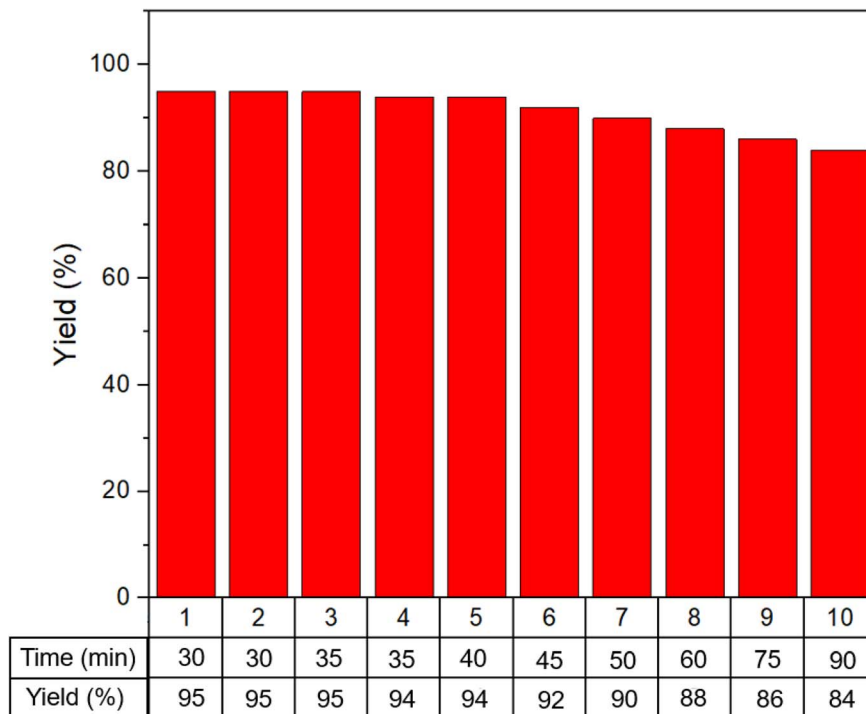
Fig. 10 Recoverability and reusability of \text{Fe}_3\text{O}_4@\text{MCM-41}@UiO-66/\text{SB-Pd} .
