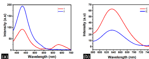
Fig. 8 PL emission spectra of DCDs in DI water–LD solution at (a) 360 nm and (b) 560 nm excitation wavelengths. 1 represents emission taken from DCDs in DI water, and 2 represents emission taken from the lipid-rich region.
