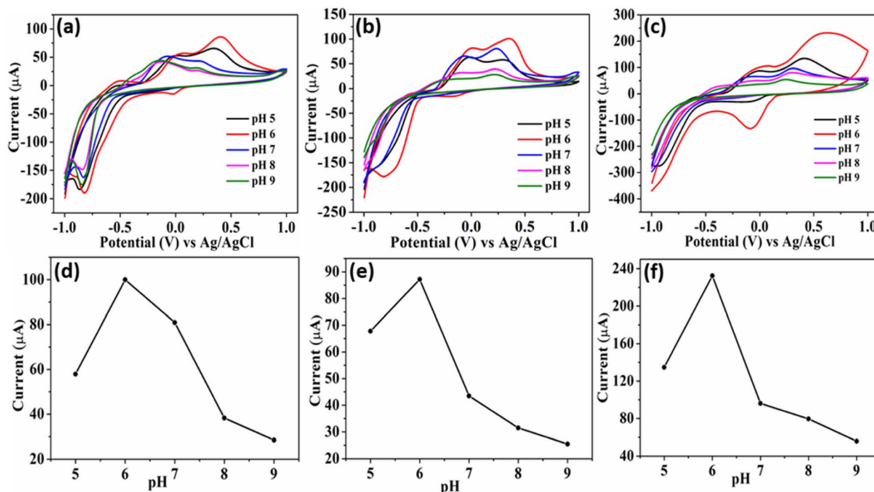
Fig. 5 CV of Cu 3 BiS 3 for 100 μM 4-NP at different 0.1 M PBS pH (5–9) (a) Cu 3 BiS 3 -sphere, (b) Cu 3 BiS 3 -rod, and (c) Cu 3 BiS 3 -worm. (d–f) The corresponding plots of current vs. different pH.
