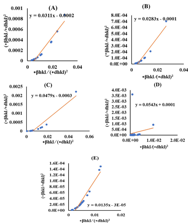
Fig. 7 HWM for (A) succinic acid_HAp, (B) ascorbic acid_HAp, (C) stearic acid_HAp, (D) calcium phosphate_HAp and (E) silica_HAp.
