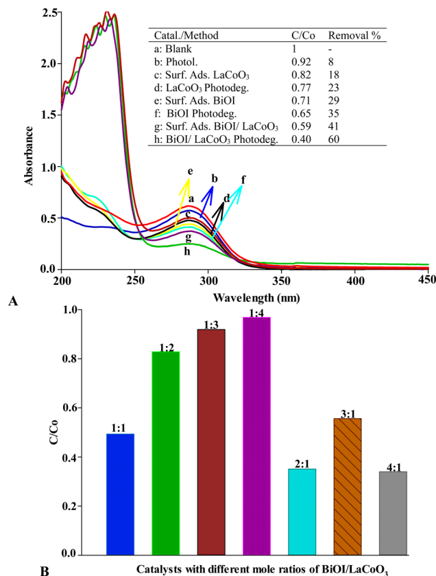
Fig. 5 (A) UV-Vis CEF absorption spectra over the applied removal processes ( 0.3 \text{ g L}^{-1} of each catalyst in 10 \text{ mL} of 10 \text{ mg L}^{-1} CEF solution, time: 40 \text{ min} , the mole ratio of BiOI : LaCoO 3 was 1 : 1 ); (B) the effect of the variation in the BiOI:LaCoO 3 molar ratio of the coupled catalyst on the CEF photodegradation.
