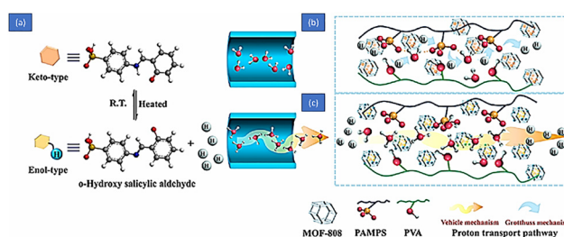
Fig. 7 Thermal-response proton transfer pathway of (a) H 2 L 23 @MOF-808 composite and their hybrid membrane (b) and (c) using the keto and enol type structure of o-hydroxy salicylaldehyde; reproduced from ref. 34 with permission from ACS, Copyright 2023.
