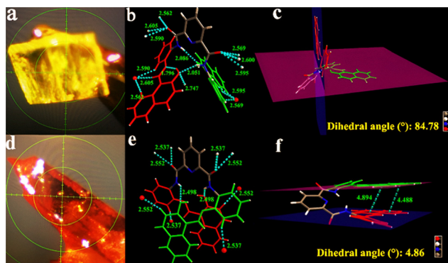
Fig. 2 Crystal photographs (a) and (d), hydrogen bonding (b) and (e), and dihedral angle (c) and (f) of H_4L^2-\gamma and H_4L^2-r Crystal, respectively; reproduced from ref. 57 with permission from RSC, Copyright 2022.
