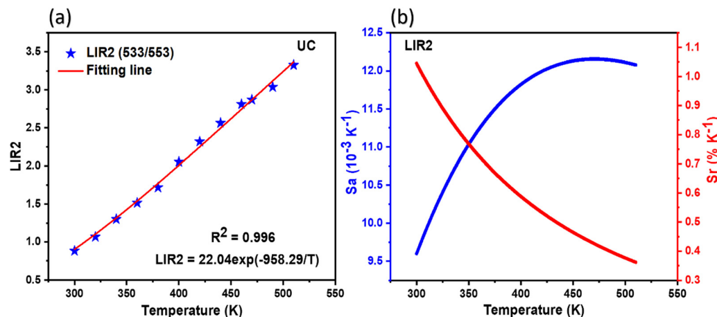
Fig. 10 (a) and (b) Temperature dependence of the LIR2 value between ^2\text{H}_{11/2} and ^4\text{S}_{3/2} TCL of \text{Er}^{3+} ions, and (b) the calculated S_r and S_a by LIR2 from TCL based on up-conversion.
