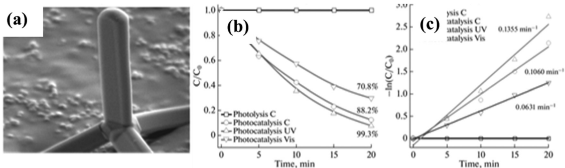
Fig. 9 (a) SEM image of ZnO TPs (b) curves of the photocatalytic degradation of MO under UV-vis, visible, and direct solar light and (c) determination of the reaction rate constant ( k , min -1 ) [Reprinted with permission from ref. 79 Copyright 2023, Springer Nature].
