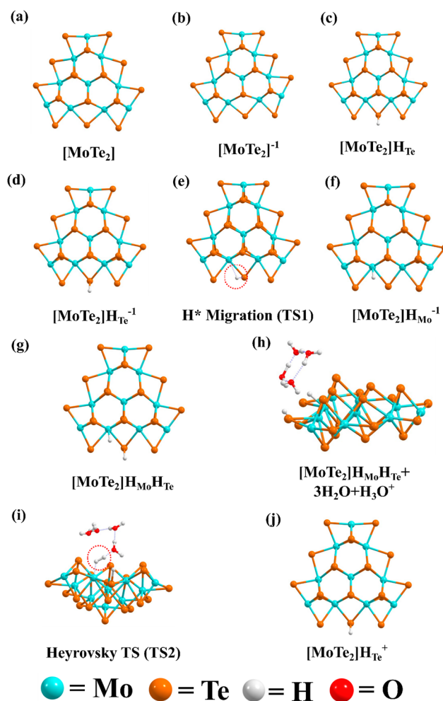
(1) The [\text{MoTe}_2] material can be found in its most stable state with a neutral Mo-edge under typical circumstances of the standard hydrogen electrode (SHE) at \text{pH} = 0 , which serves as the starting point for our estimates of the thermodynamic potential. [\text{MoTe}_2] represents the abbreviation for the finite molecular cluster \text{Mo}_{10}\text{Te}_{21} . Fig. 4a shows the equilibrium structure of the [\text{MoTe}_2] material.
