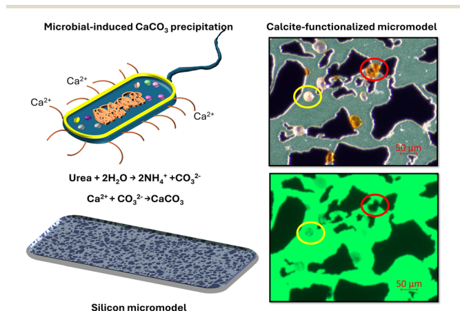
Fig. 1 Design and characterization of calcite-functionalized micromodels. This schematic illustration depicts the fabrication process of calcite-functionalized micromodels via microbial-induced carbonate precipitation. The right column shows microscopy images of deposited calcite precipitates within the pore network, captured in bright-field (top) and fluorescence (bottom) channels. Calcite precipitates are categorized into two types: partial growth that restricts flow (highlighted by yellow circles) and complete growth that blocks flow (indicated by red circles).
