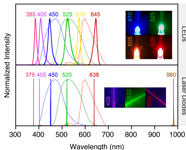
Fig. 5 LEDs and laser diodes. Examples of emission spectra of LEDs (top) and laser diodes (bottom) superimposed on the average spectral responses of the smartphone camera RGB color channels (dotted lines). The insets show images of LEDs and beams from laser diodes. Some digital adjustment of color was made to these images to mimic the appearance to the human eye. LED and laser diode spectra were plotted from publicly available vendor data (ThorLabs) for commercial products.
