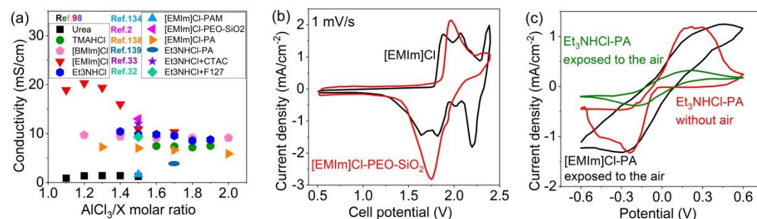
Figure 15. a) Ionic conductivity of various \text{AlCl}_3/\text{X} electrolytes. \text{X} = [\text{EMIm}]\text{Cl} ( 10\text{--}20\text{ mS cm}^{-1} ), TMAHCl (average \sim 7.5\text{ mS cm}^{-1} ), Et 3 NHCl ( \sim 9.6\text{ mS cm}^{-1} ), [BMIm]Cl ( \sim 9.4\text{ mS cm}^{-1} ), and urea ( \sim 1.3\text{ mS cm}^{-1} ) were measured at 25\text{ }^\circ\text{C} . 98 [EMIm]Cl-PAM ( 1.66 \times 10^{-3}\text{ S cm}^{-1} , measured at 20\text{ }^\circ\text{C} ) is gel polymer electrolyte made from \text{AlCl}_3 complexed acrylamide and \text{AlCl}_3/[\text{EMIm}]\text{Cl} (1.5:1). 134 [EMIm]Cl-PEO-SiO 2 ( 13\text{ mS cm}^{-1} ) is gel polymer electrolyte made from PEO, \text{AlCl}_3/[\text{EMIm}]\text{Cl} (1.5:1) and an additive-fumed SiO 2 . 2 [EMIm]Cl-PA ( 5.89\text{ to }7.24\text{ mS cm}^{-1} , measured at room temperature) and Et 3 NHCl-PA ( 3.86\text{ mS cm}^{-1} , measured at 25\text{ }^\circ\text{C} ) is PA-based gel polymer electrolyte made with \text{AlCl}_3/[\text{EMIm}]\text{Cl} (2:1 to 1.3:1) 138 and \text{AlCl}_3/\text{Et}_3\text{NHCl} (1.7:1) 139 , respectively. \text{AlCl}_3/\text{Et}_3\text{NHCl} (1.5:1) add CTAC ( 12.06\text{ mS cm}^{-1} ) 33 and F127 ( 9.31\text{ mS cm}^{-1} ) 32 are named Et 3 NHCl+CTAC and Et 3 NHCl+F127, respectively. b) CV curves of Al/natural graphite cells with \text{AlCl}_3/[\text{EMIm}]\text{Cl} and \text{AlCl}_3/[\text{EMIm}]\text{Cl-PEO-SiO}_2 electrolytes showing anions intercalation at a scan rate of 1\text{ mV s}^{-1} . Adapted from Leung, O. M. et al, Adv. Energy Mater. 2 . Licensed under CC BY 3.0. ©2024 John Wiley and Sons. c) CV curves of Al/natural graphite cells with \text{AlCl}_3/[\text{EMIm}]\text{Cl-PA} 138 (not mentioning the scan rate) and \text{AlCl}_3/\text{Et}_3\text{NHCl-PA} 139 (without air not mentioning the scan rate, and after being exposed to the air for 10 min at a scan rate of 1\text{ mV s}^{-1} ) presenting Al plating/stripping. Adapted with permission from Elsevier 138 . Copyright 2021. Adapted with permission from American Chemical Society 139 . Copyright 2021.
