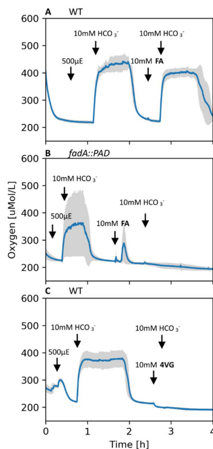
Fig. 1 Oxygen measurement of Synechococcus sp. PCC11901 in the presence of ferulic acid (FA) and 4-vinyl guaiacol (4VG). Measurement was taken in a closed vessel, prohibiting \text{CO}_2 from entering the suspension. The cell density was set to 3.9 gDCW \text{L}^{-1} . Light intensity was increased to 500 \mu\text{mol photons m}^{-2} \text{ s}^{-1} until \text{O}_2 stagnated, and then 10 mM of a carbonate solution was added, causing a spike in \text{O}_2 concentration. Then, 10 mM of either ferulic acid (A, B) or 4-vinyl guaiacol (C) was added, followed by another addition of carbonate and the oxygen levels were compared. (A) WT strain with 10 mM ferulic acid (B) fadA::pad strain with 10 mM ferulic acid and (C) WT with 10 mM 4-vinyl-guaiacol. The grey area indicates the standard error of the mean from 3 replicates.
