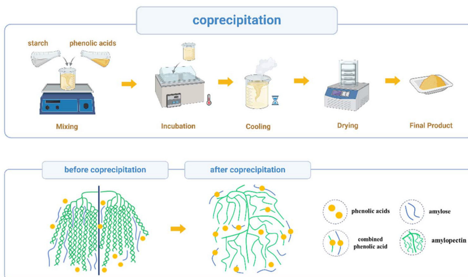
Fig. 4 Preparation of starch–phenolic acid complexes via coprecipitation and the associated structural modifications.
