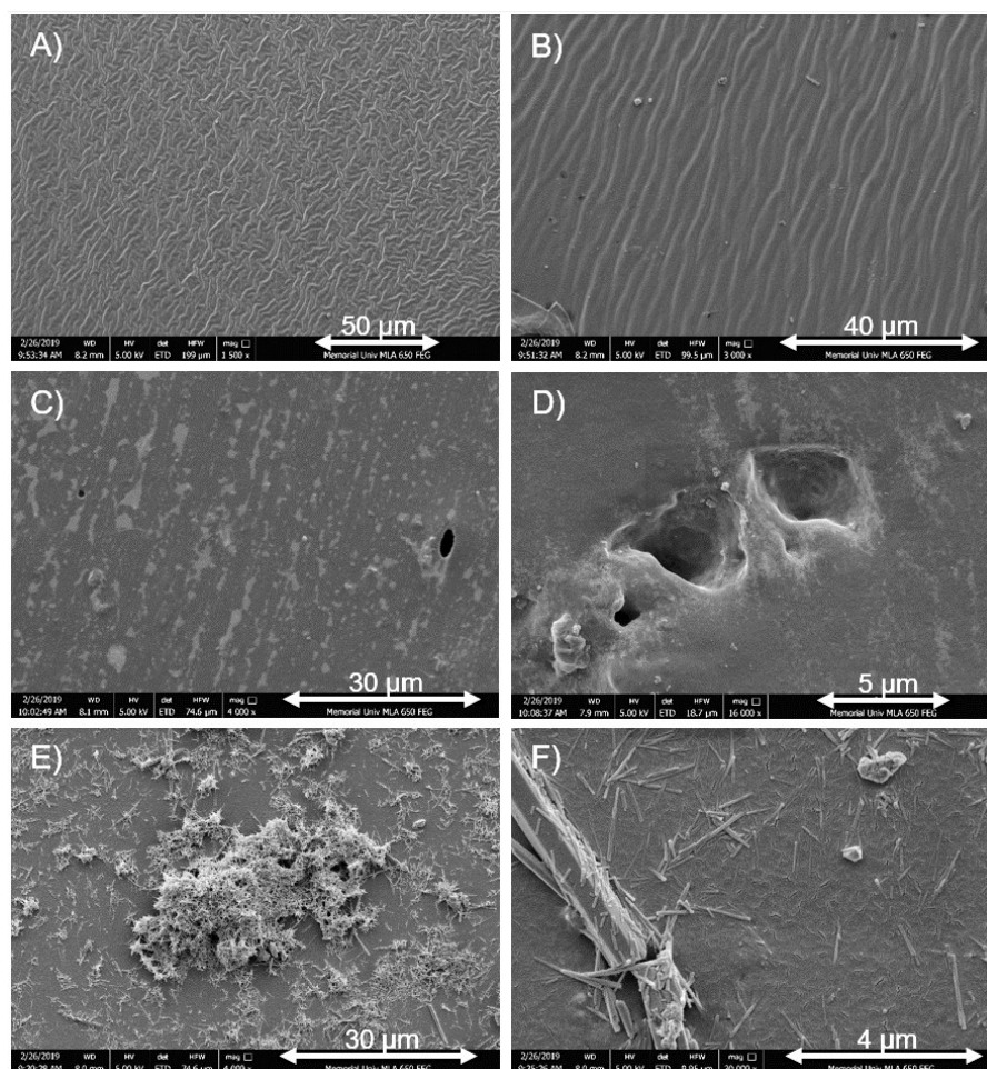
Figure 2: Selected, typical SEM images of FO-NIPU films exposed to water for 28 days, A-B) original film, C-D) deionized water NIPU film, and E-F) synthetic sea water NIPU film.
