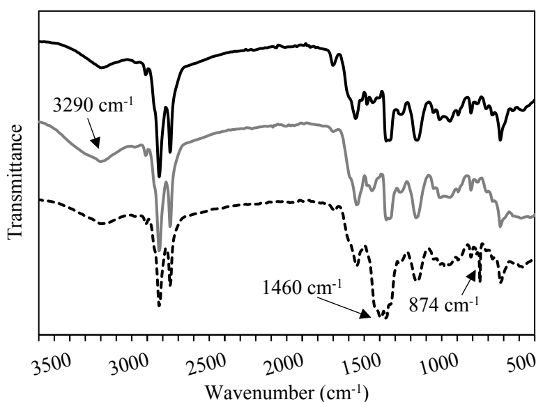
Figure 6: IR spectra of FO-NIPU (black, top), deionized water NIPU (gray, middle), and seawater-exposed FO-NIPU (black dashed, bottom).
