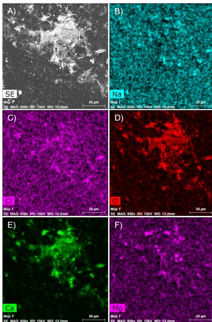
Figure 4: SEM-EDX elemental maps of crystalline material found on the surface of the FO-NIPU film after exposure to synthetic sea water. A) SEM image of agglomerate and elemental maps of B) sodium, C) chlorine, D) oxygen, E) calcium, and F) magnesium.
