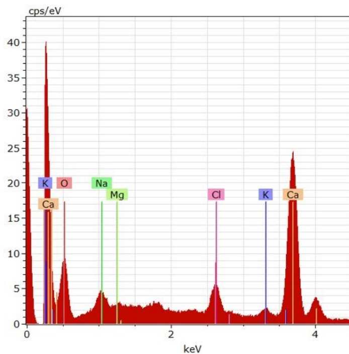
Figure 3: EDX spectrum of crystals on film exposed to synthetic sea water.
