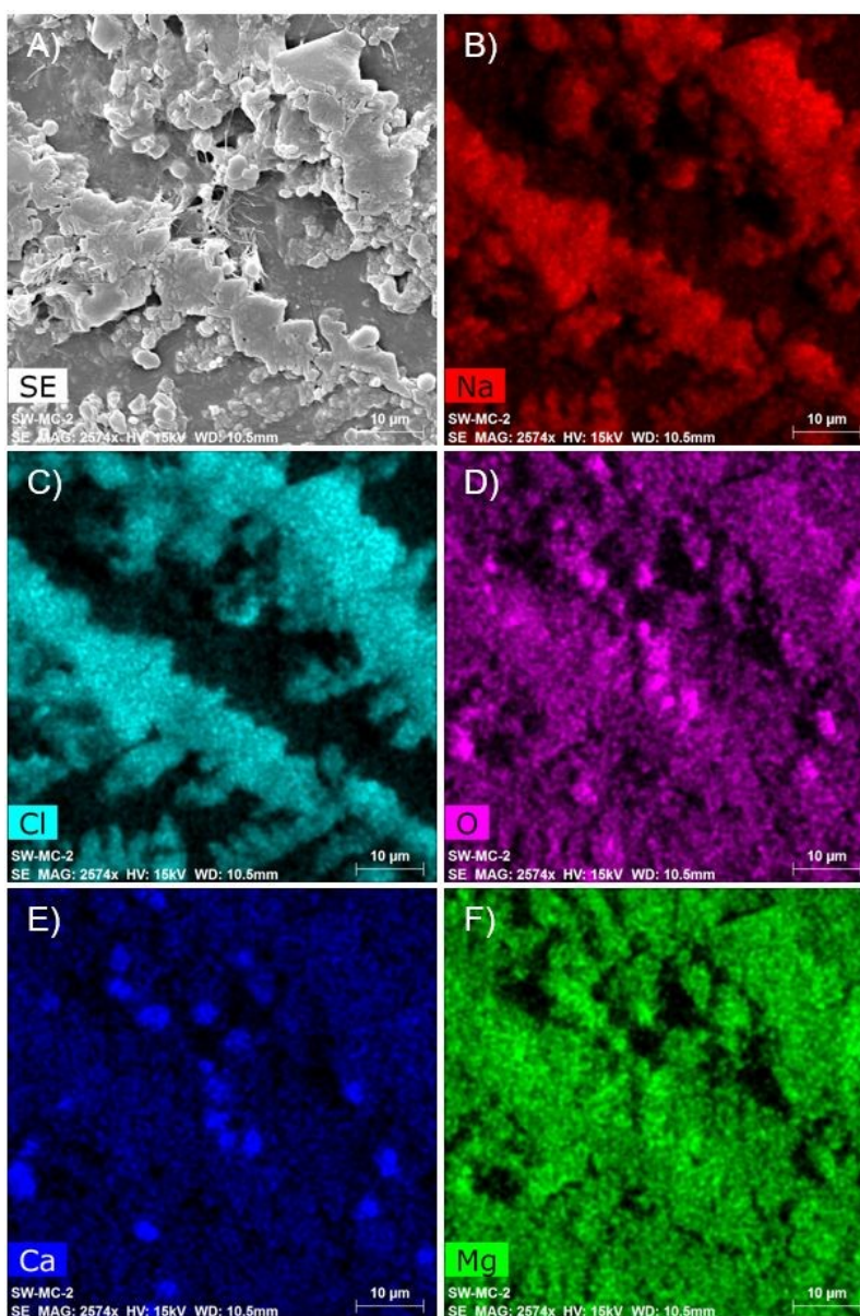
Figure 5: SEM image of the surface of FO-NIPU film exposed to Middle Cove seawater A) and elemental maps of B) sodium, C) chlorine, D) oxygen, E) calcium, and F) magnesium.
