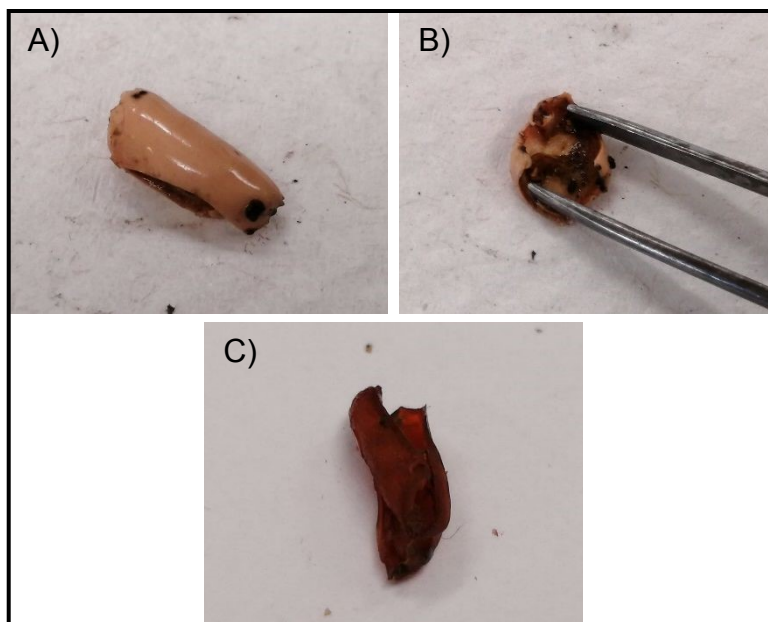
Figure 8: Images of degraded NIPU film. A) and B) show film after removal from solution and C) after drying in air overnight.
