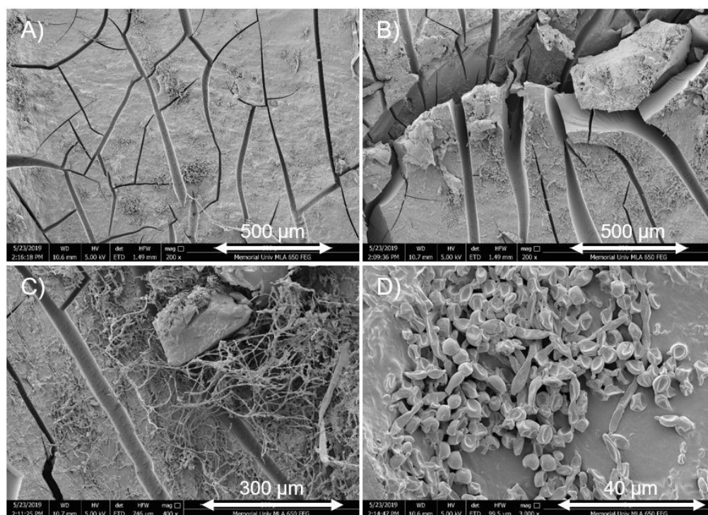
Figure 9: SEM images of degraded NIPU film. A) and B) surface of film, C) mold hyphae, and D) clusters of bacteria on surface.
